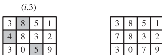
Figure 15.1: An item comes in, and 3 is to be added to the count. The initial state is on the left; the shaded counters need to be updated. Using conservative update, the minimum counter value 4 determines that all corresponding counters need to be pushed up to at least 4 + 3 = 7 . The resulting state after the update is shown on the right.
