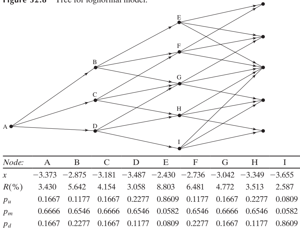
Figure 32.8 Tree for lognormal model.
