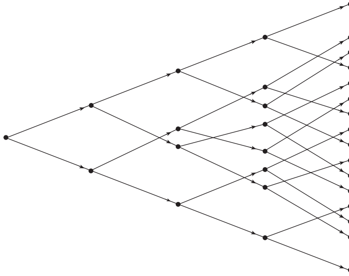
Figure 33.1 A nonrecombining tree such as that arising from the general HJM model.
