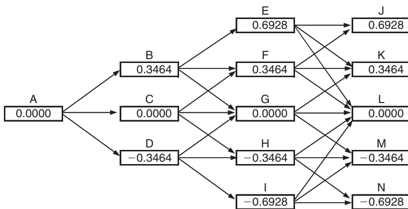
Figure 35.1 Tree for X . Constructing this tree is the first stage in constructing a tree for the spot price of a commodity, S . Here p_u , p_m , and p_d are the probabilities of “up”, “middle”, and “down” movements from a node.
