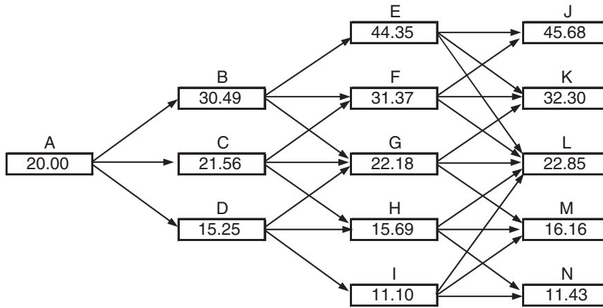
Figure 36.1 Tree for spot price of a commodity: p_u, p_m, and p_d are the probabilities of “up”, “middle”, and “down” movements from a node.
