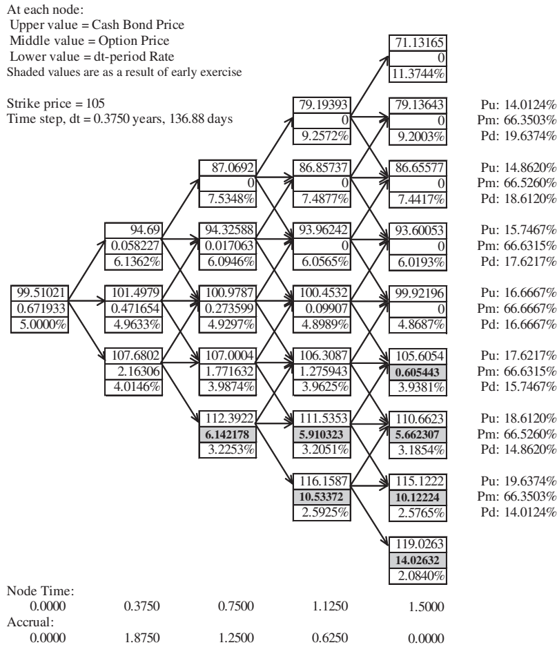
Figure 32.9 Tree, produced by DerivaGem, for valuing an American bond option.
