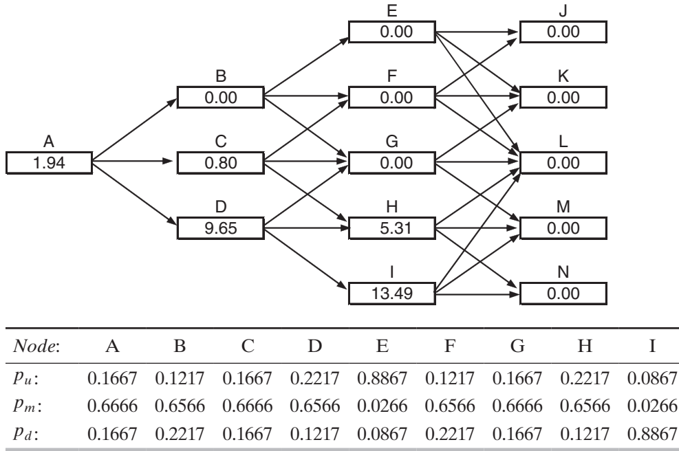
Figure 36.3 Valuation of option to abandon the project: p_u , p_m , and p_d are the probabilities of “up”, “middle”, and “down” movements from a node.
