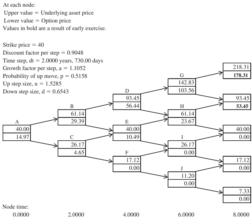
Figure 16.1 Valuation of employee stock option in Example 16.2.
