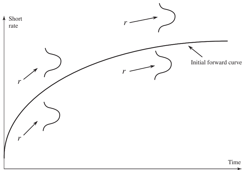
Figure 32.1 The Ho–Lee model.
