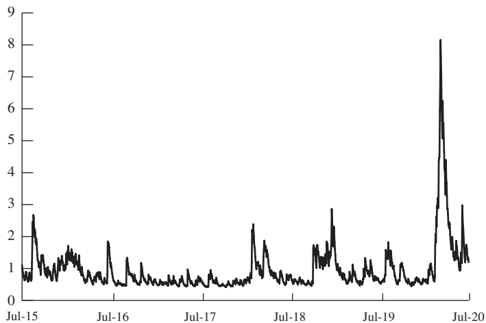
Figure 23.2 Volatility (% per day) of S&P 500 index: July 10, 2015, to July 9, 2020.
