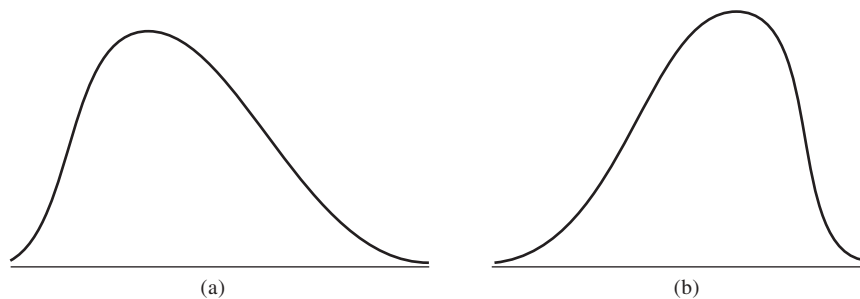
Figure 22.3 Probability distribution for value of portfolio: (a) positive gamma; (b) negative gamma.
