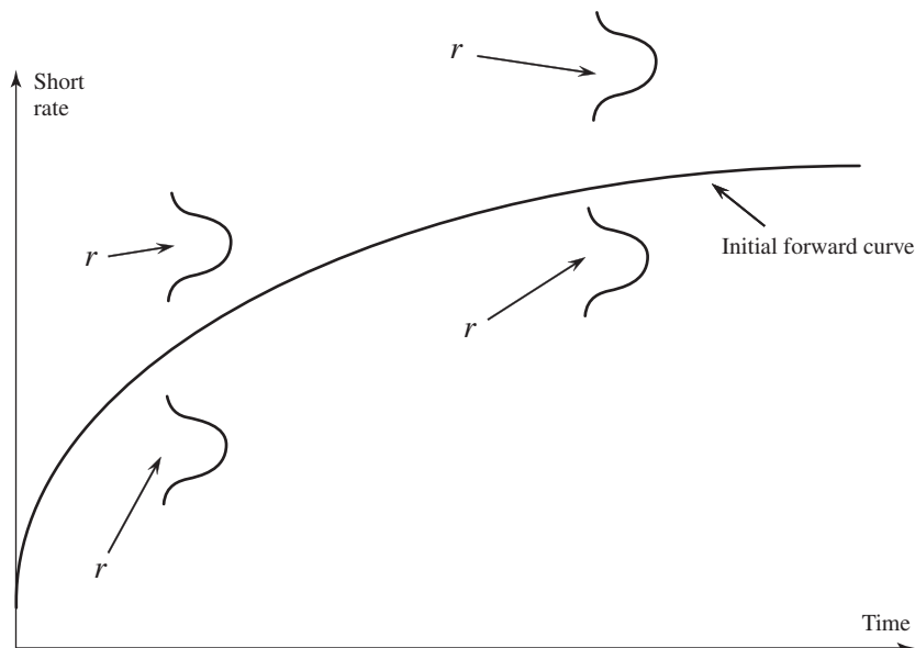
Figure 32.2 The Hull–White model.
