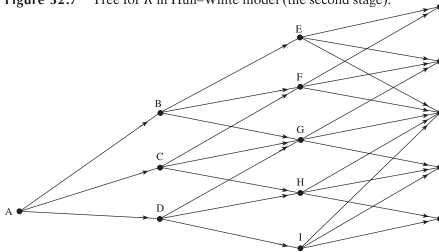
Figure 32.7 Tree for R in Hull–White model (the second stage).
