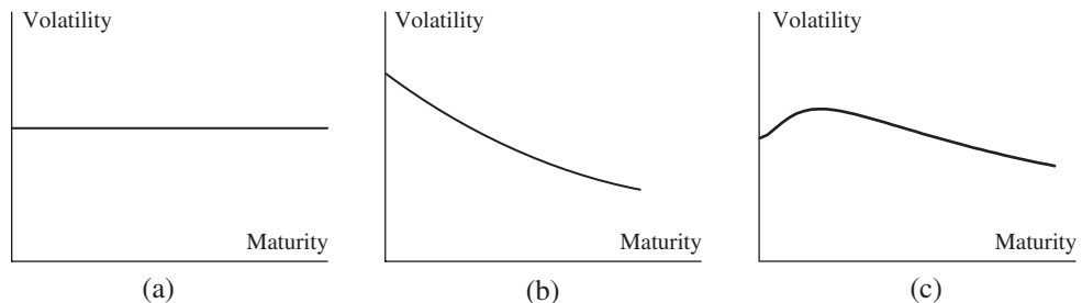
Figure 32.3 Volatility of 3-month forward rate as a function of maturity for (a) the Ho–Lee model, (b) the Hull–White one-factor model, and (c) the Hull–White two-factor model (when parameters are chosen appropriately).
