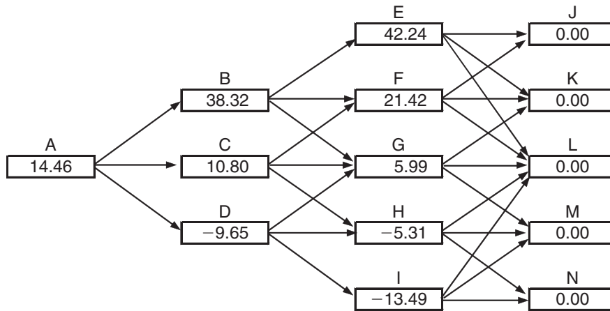
Figure 36.2 Valuation of base project with no embedded options: p_u , p_m , and p_d are the probabilities of “up”, “middle”, and “down” movements from a node.
