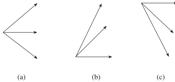
Figure 32.5 Alternative branching methods in a trinomial tree.
