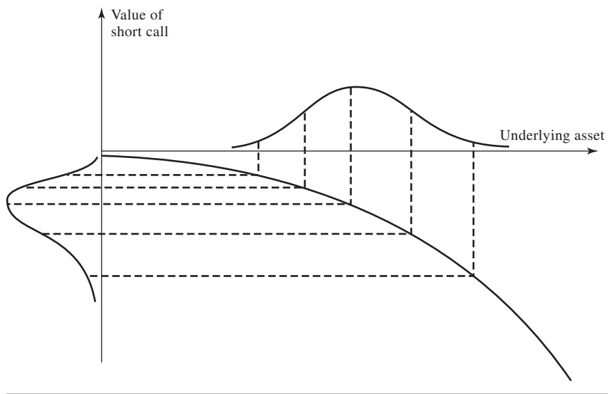
Figure 22.5 Translation of normal probability distribution for asset into probability distribution for value of a short call on asset.
