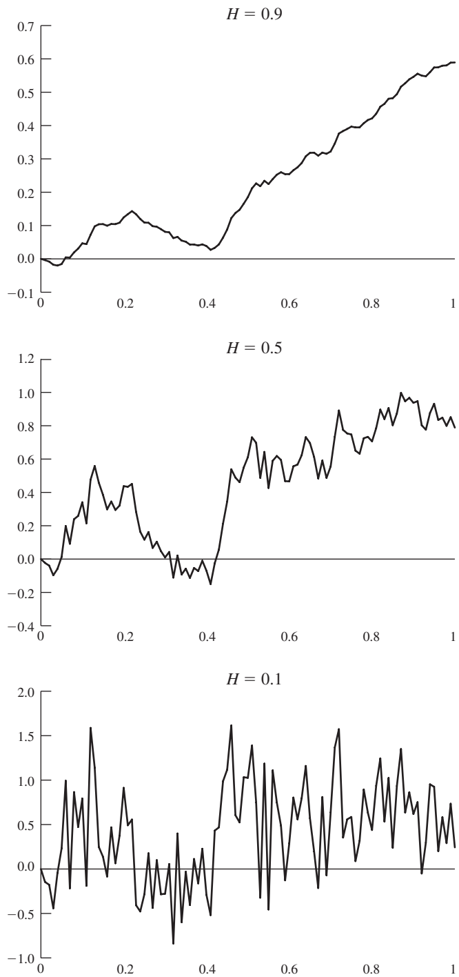
Figure 14.3 Simulation of fractional Brownian motion for different values of the Hurst exponent.
