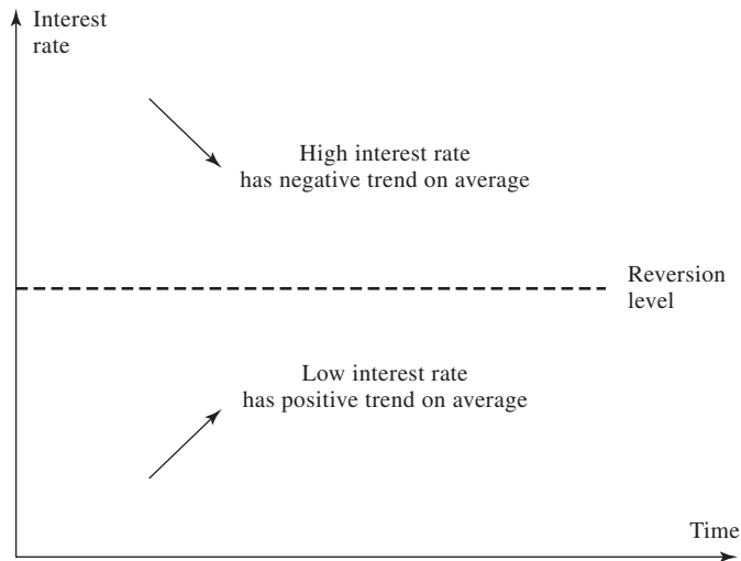
Figure 31.1 Mean reversion.
