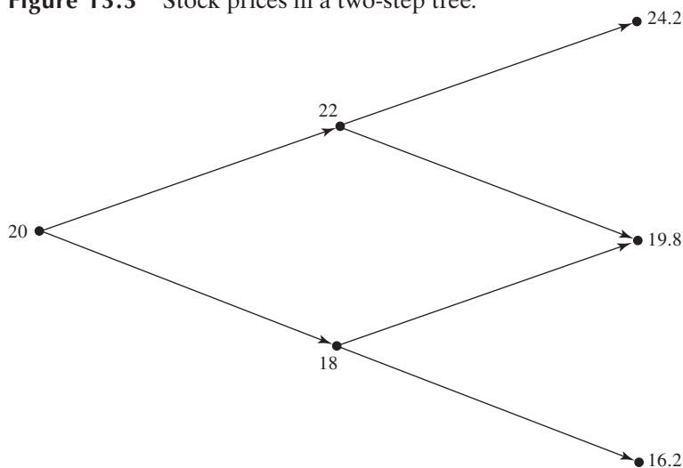
Figure 13.3 Stock prices in a two-step tree.
