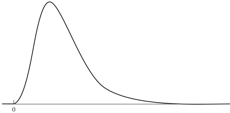
Figure 15.1 Lognormal distribution.
