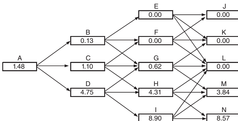
Figure 35.3 Valuation of an American put option with a strike price of $20 using the tree in Figure 35.2.
