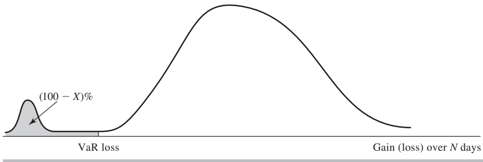
Figure 22.2 Alternative situation to Figure 22.1. VaR is the same, but the potential loss is larger.
