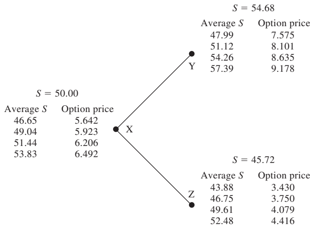
Figure 27.3 Part of tree for valuing option on the arithmetic average.
