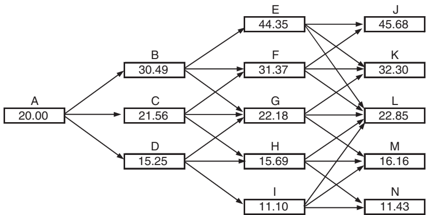
Figure 35.2 Tree for spot price of a commodity: p_u , p_m , and p_d are the probabilities of “up”, “middle”, and “down” movements from a node.
