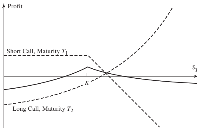
Figure 12.8 Profit from calendar spread created using two call options, calculated at the time when the short-maturity call option expires.
