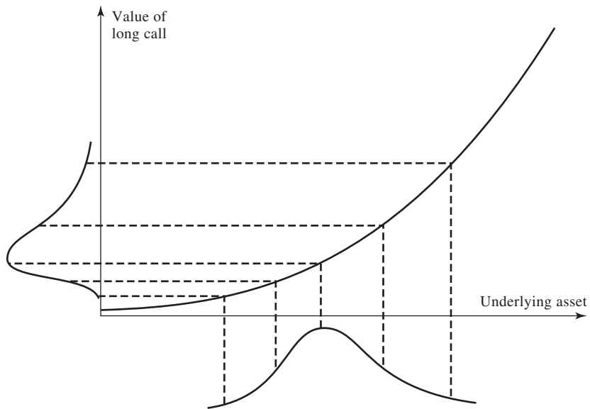
Figure 22.4 Translation of normal probability distribution for asset into probability distribution for value of a long call on asset.
