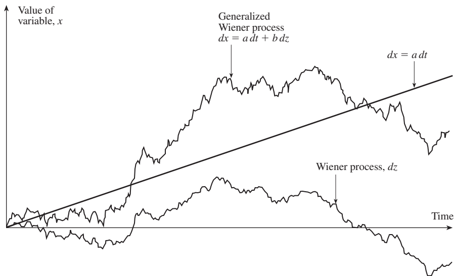
Figure 14.2 Generalized Wiener process with a = 0.3 and b = 1.5 .
