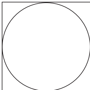
Figure 21.13 Calculation of \pi by throwing darts.
