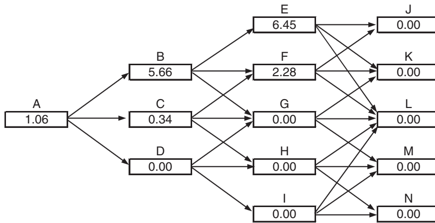
Figure 36.4 Valuation of option to expand the project: p_u , p_m , and p_d are the probabilities of “up”, “middle”, and “down” movements from a node.
