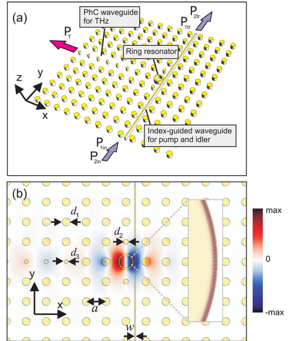
FIG. 1. (Color online) (a) Schematic of the triply-resonant nonlinear photonic structure analyzed in the text. P_{\text{in}} and P_{\text{2in}} denote the input powers at the pump and idler frequencies, respectively; whereas P_{\text{1tr}} and P_{\text{2tr}} represent the corresponding transmitted powers through the structure. P_T stands for the THz output power. (b) Main panel: Electric field profile ( E_z ) corresponding to the resonant mode appearing at 1 THz in the structure shown in (a). The value of the different geometrical parameters displayed in this figure are a=102 \mu\text{m} , d_1=40.8 \mu\text{m} , d_2=25.1 \mu\text{m} , d_3=18.8 \mu\text{m} , and w=0.8 \mu\text{m} . Inset displays an enlarged view of the electric field profile ( E_x ) corresponding to a whispering gallery with m=572 circulating inside the dielectric ring shown in the main figure. The internal and external radii defining the ring resonator are 30.5 \mu\text{m} and 40.1 \mu\text{m} , respectively. Shaded areas in both the main and inset figures represent GaAs regions, while white areas represent air.
