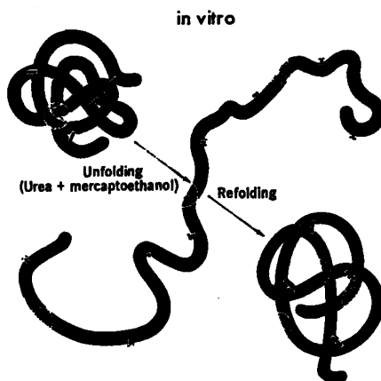
Fig. 2. Schematic representation of the redutive denaturation, in 8M urea solution containing 2-mercaptoethanol, of a disulfide-cross-linked protein. The conversion of the extended, denatured form to a randomly cross-linked, "scrambled" set of isomers is depicted at the lower right.
